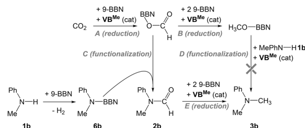
Scheme 3. Proposed pathways for the catalytic methylation of 1b with CO 2 and 9-BBN.
